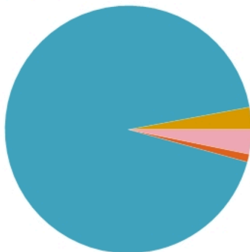
Cannabinoid Potency Chart
